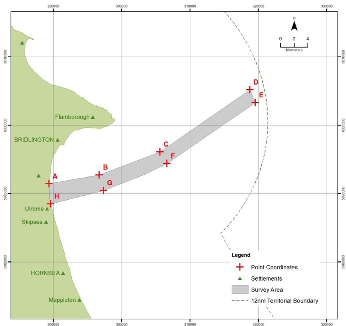
Figure 1: Above; survey area plan for near-shore geophysical survey activity – MV Titan Endeavour
