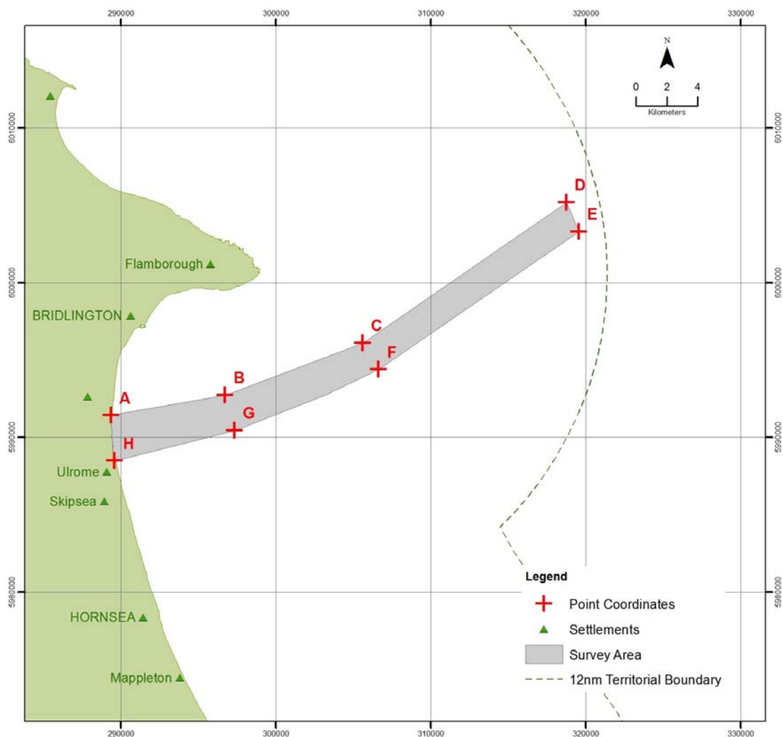
Figure 1: Above; survey area plan for near-shore environmental survey activity – MV Titan Endeavour
