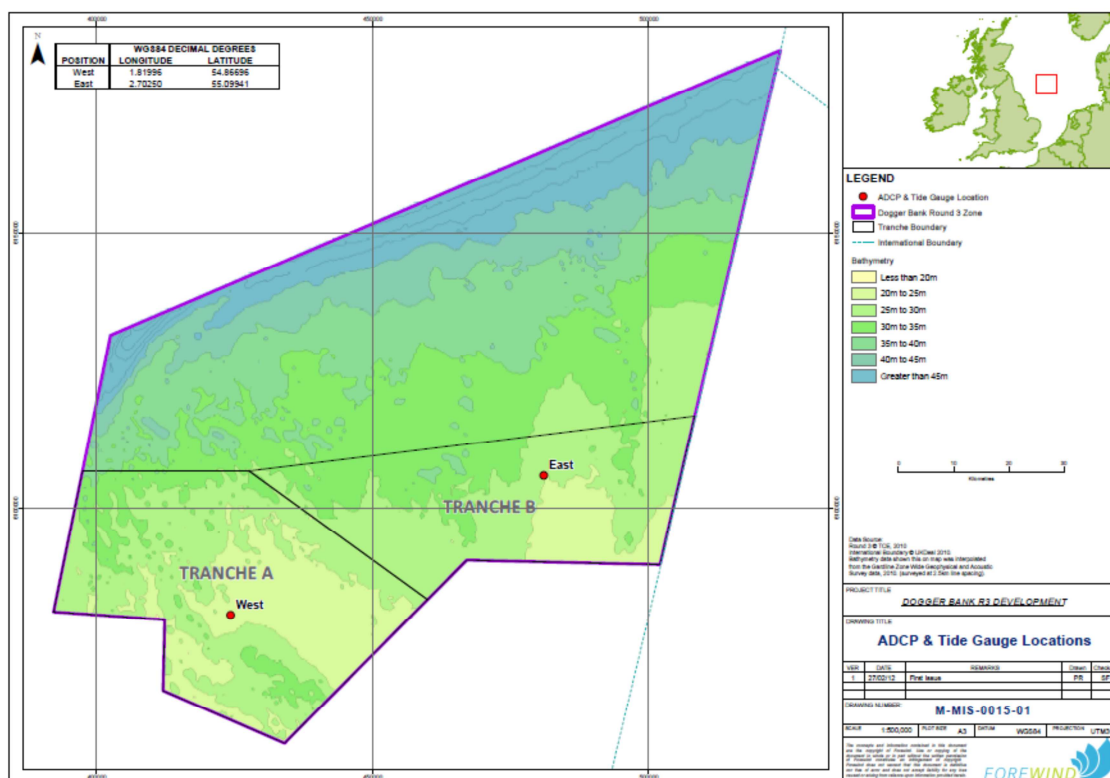
Figure 1: Above; locations of the seabed-anchored wave and current measurement devices.
